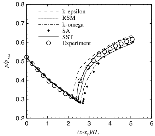
Fig. 7 Wall static pressure distribution on the large separation for A_e/A_t = 1.5 and \text{NPR} = 1.6 .
