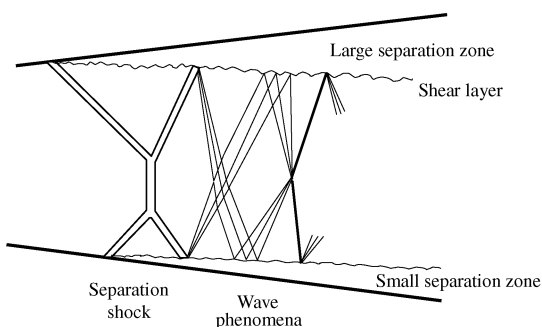
Fig. 2 Picture and sketch of principal flow features of supersonic nozzle flow separation [4].
