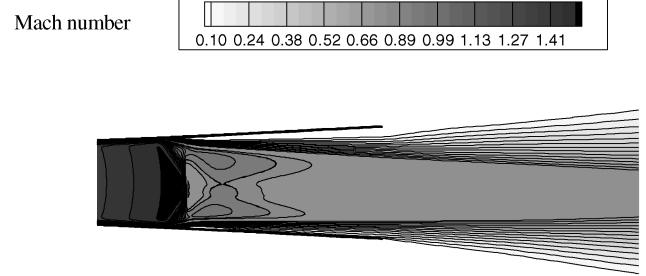
Fig. 6 Mach number contours inside and outside the nozzle for A_e/A_t = 1.5 and \text{NPR} = 1.6 .
